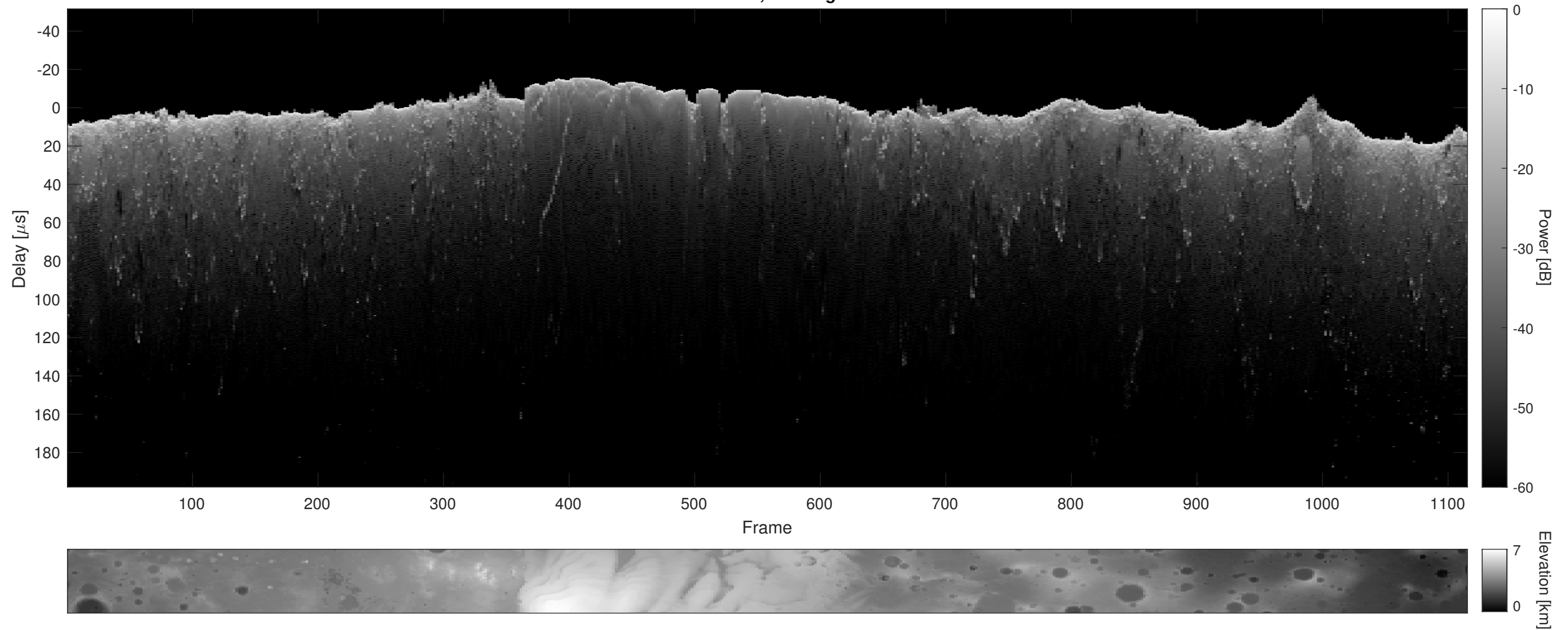
Orbit 12851, Cluttergram
