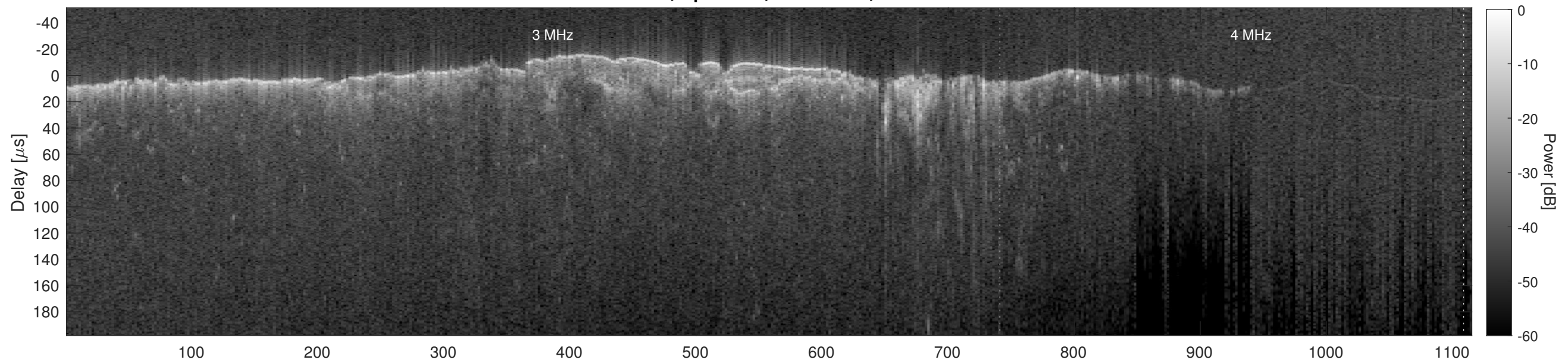
Orbit 12851, Cluttergram
