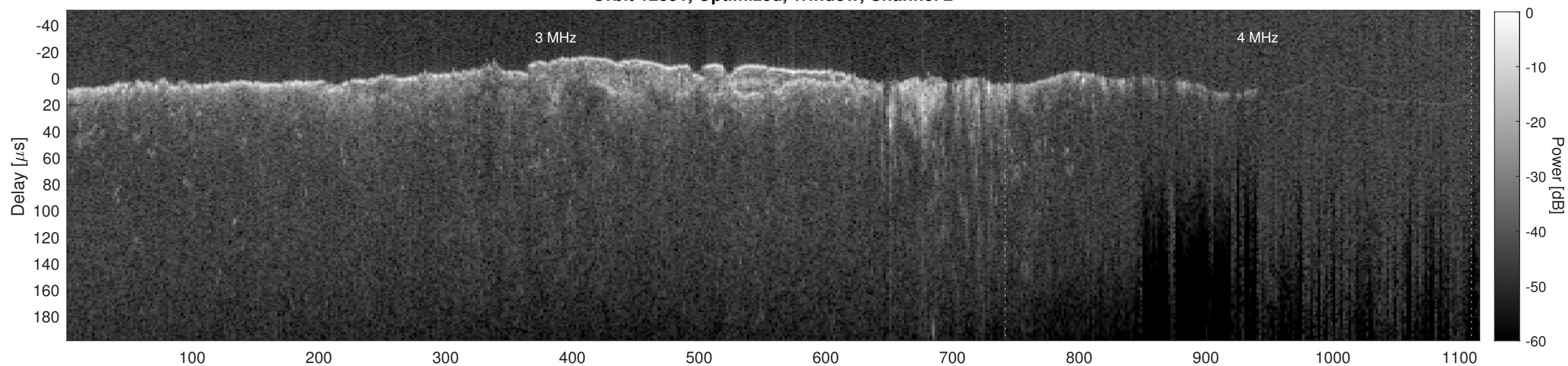
Orbit 12851, Cluttergram
