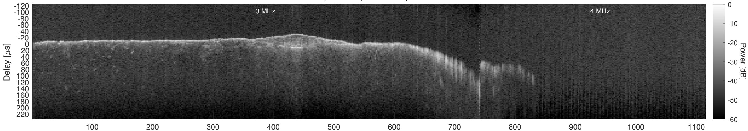
Orbit 12852, Window, Channel 2, Chapman
