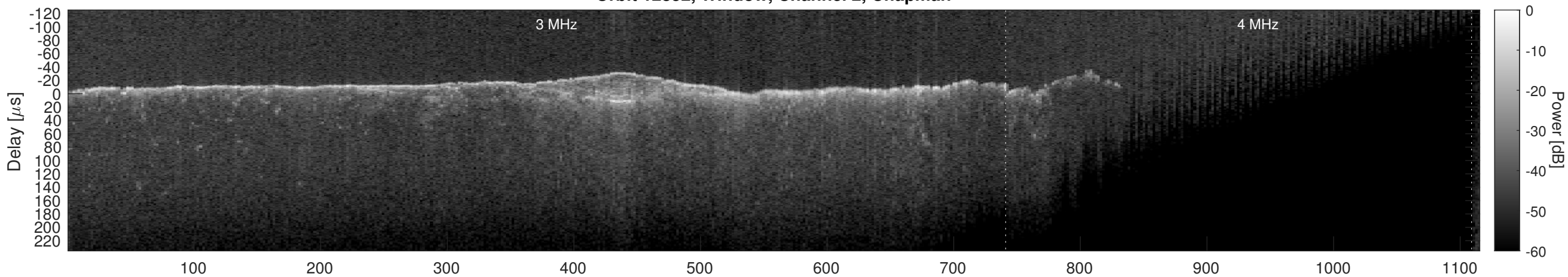
Orbit 12852, Window, Channel 2, Optimized
