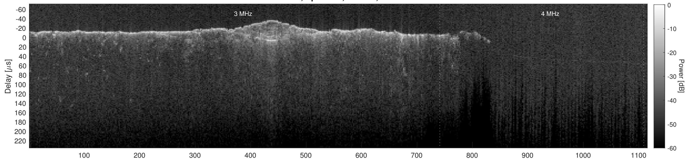
Orbit 12852, Cluttergram
