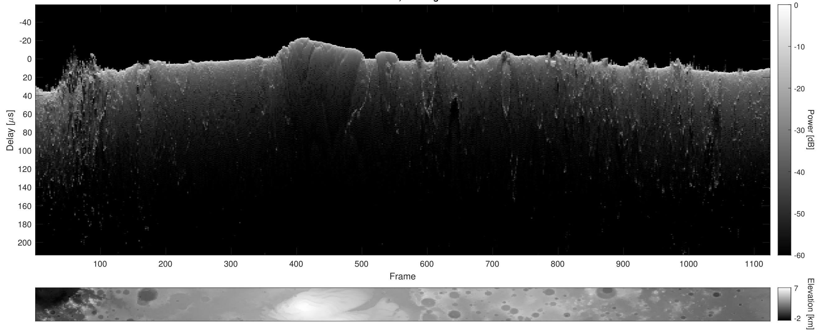
Orbit 12855, Cluttergram
