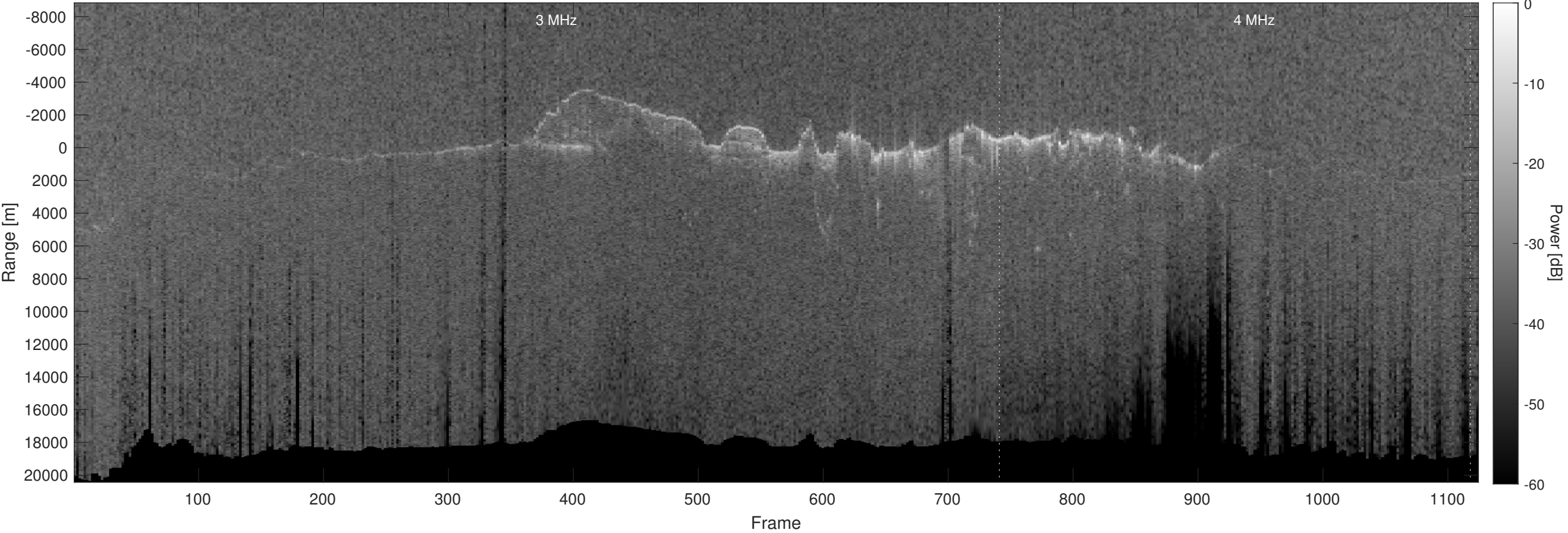
Orbit 12855, Optimized, No Window, Depth-Corrected, Channel 2
