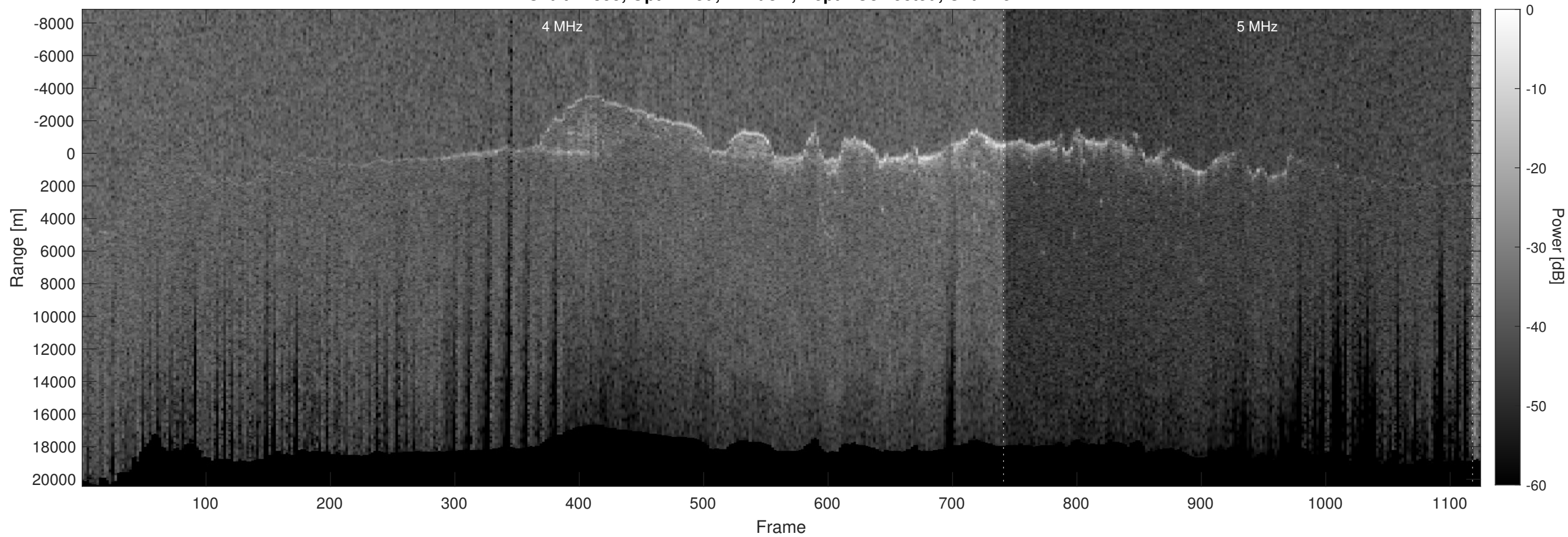
Orbit 12855, Optimized, Window, Depth-Corrected, Channel 2
