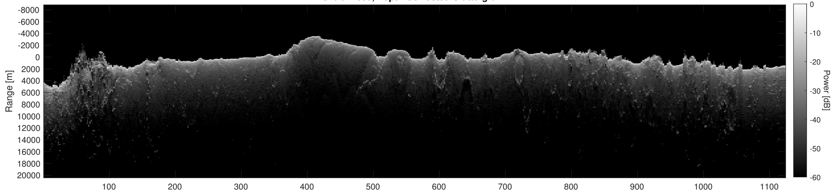
Orbit 12855, Depth-Corrected Cluttergram
