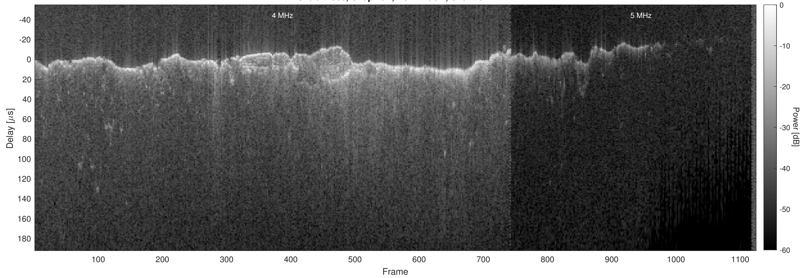
Orbit 12856, Chapman, No Window, Channel 2
