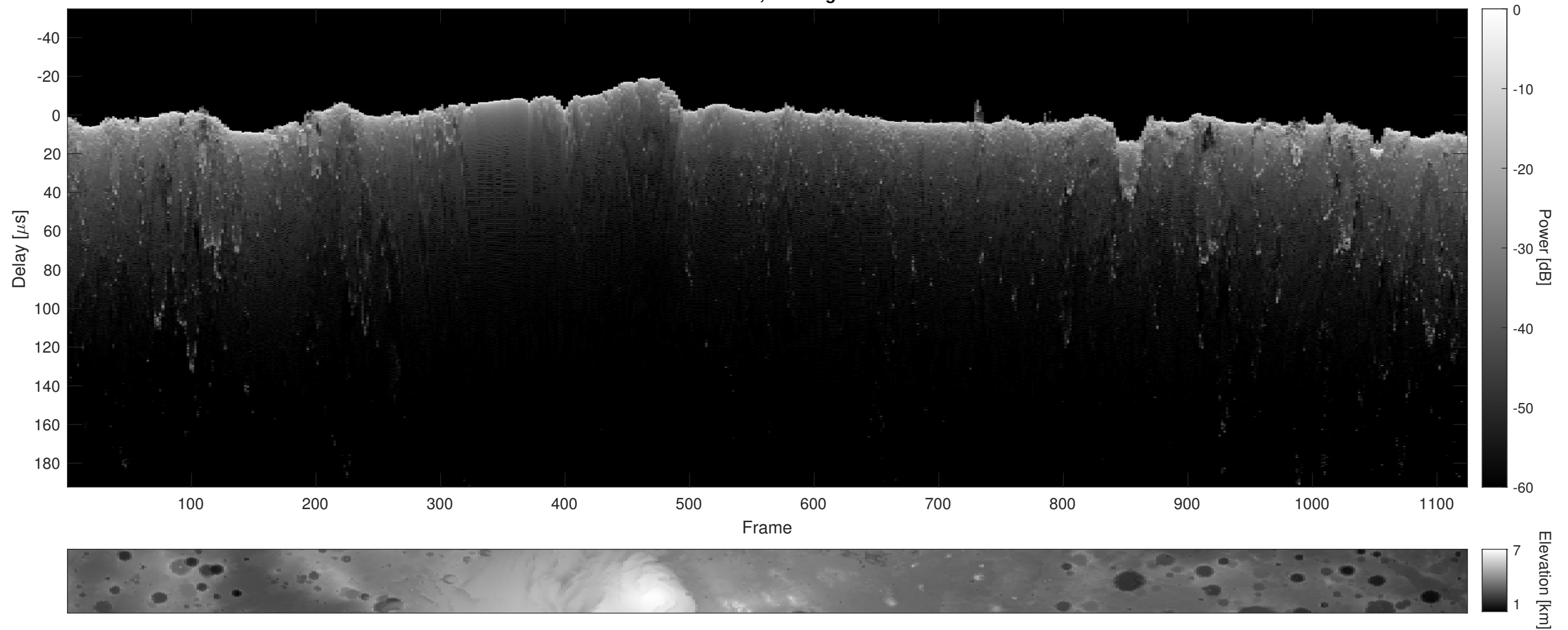
Orbit 12856, Cluttergram
