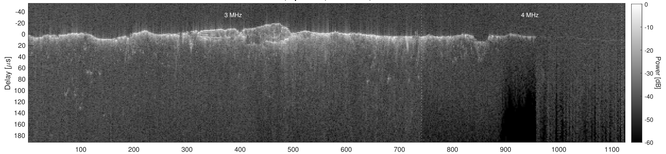
Orbit 12856, Cluttergram
