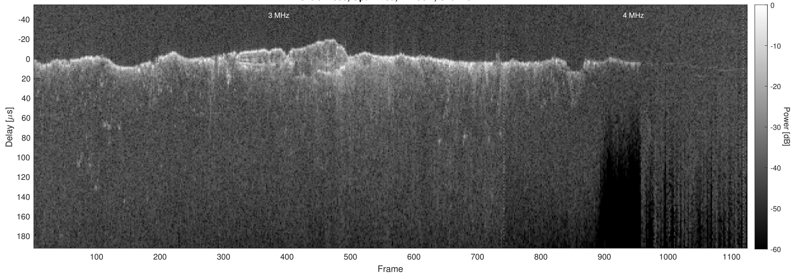
Orbit 12856, Optimized, Window, Channel 2
