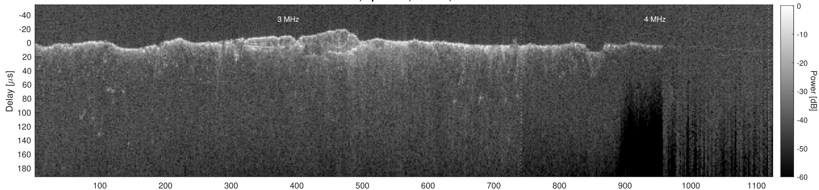
Orbit 12856, Cluttergram
