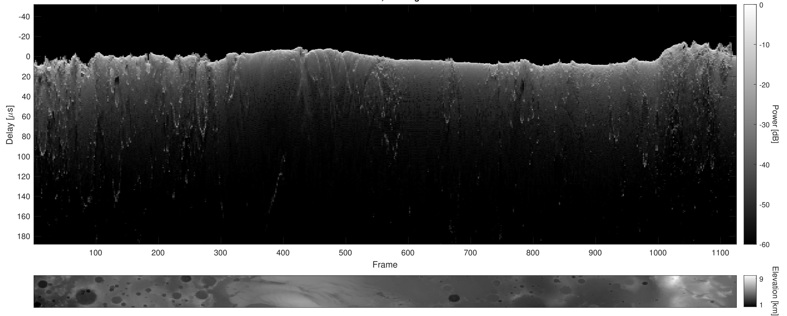
Orbit 12857, Cluttergram
