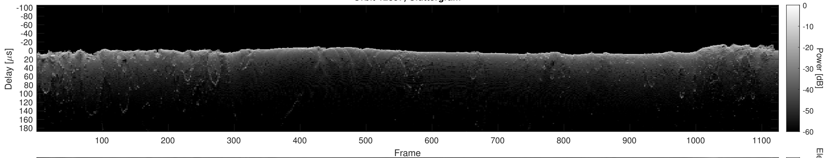
Orbit 12857, Cluttergram
