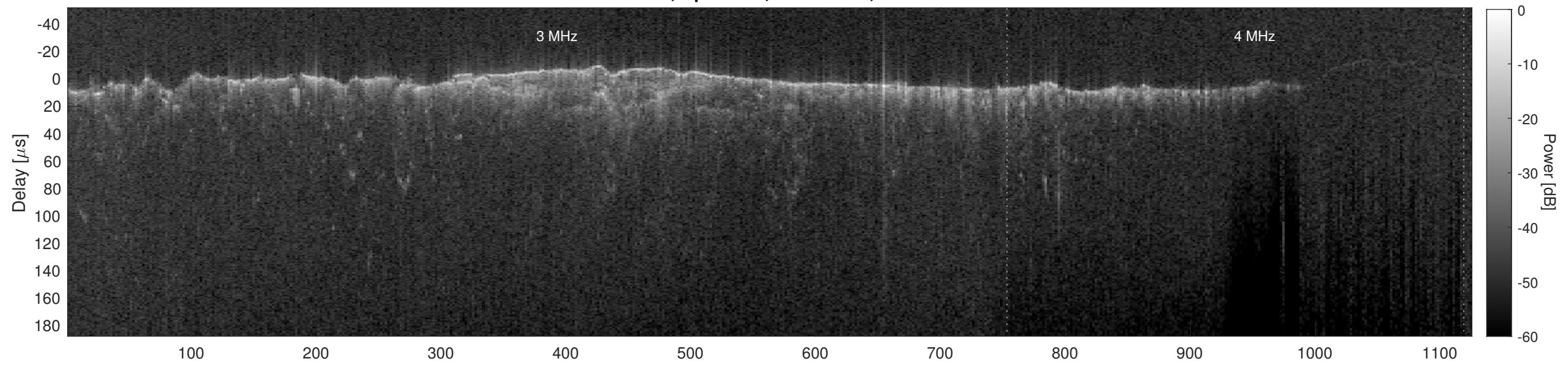
Orbit 12857, Cluttergram
