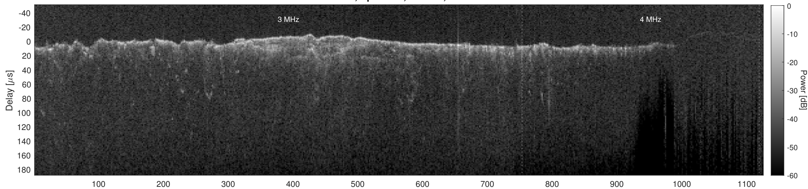
Orbit 12857, Cluttergram
