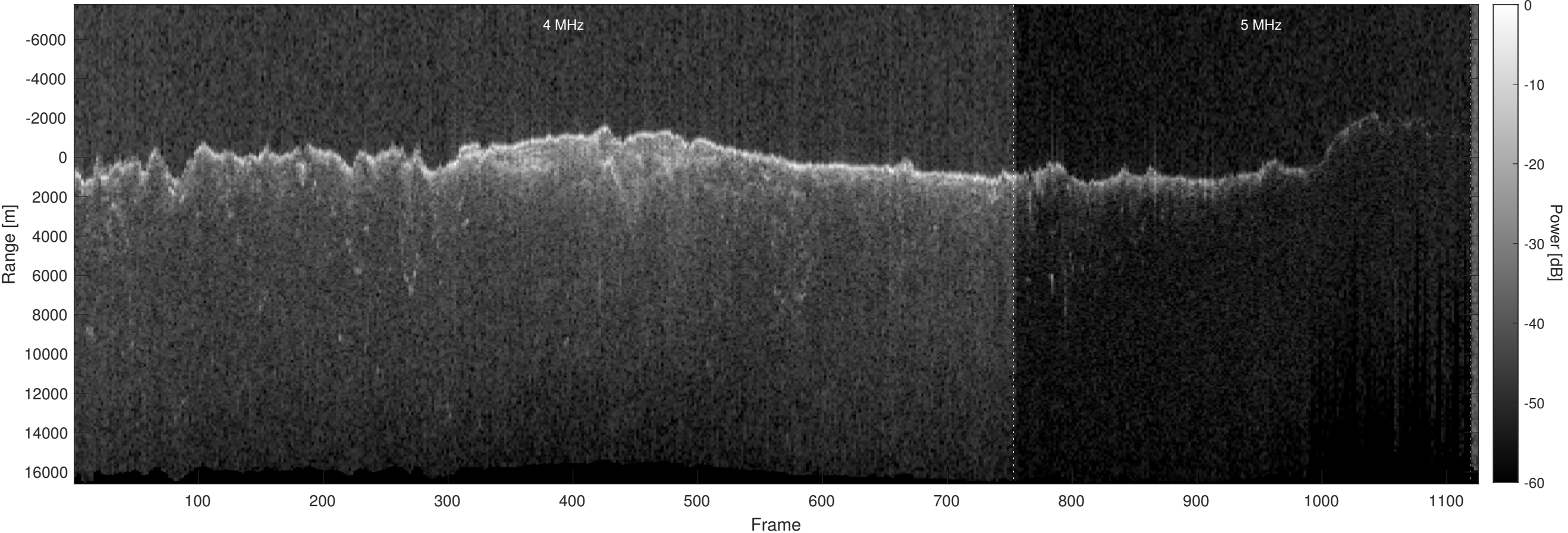
Orbit 12857, Optimized, Window, Depth-Corrected, Channel 2
