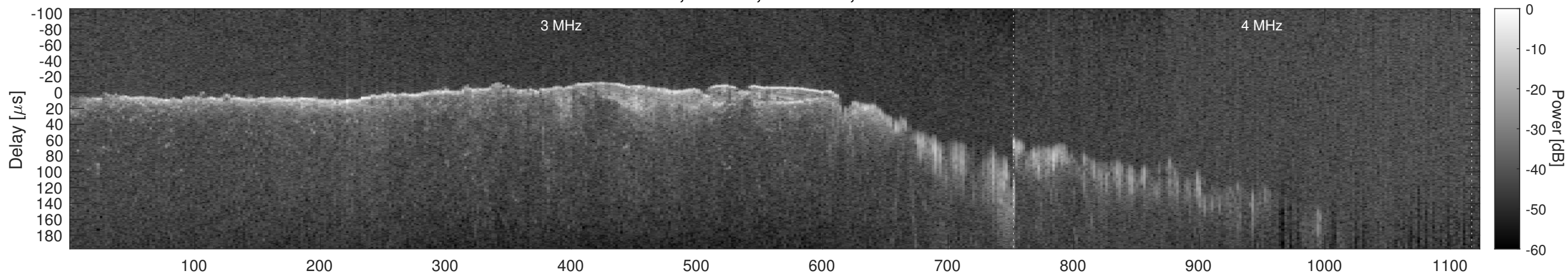
Orbit 12858, Window, Channel 2, Chapman
