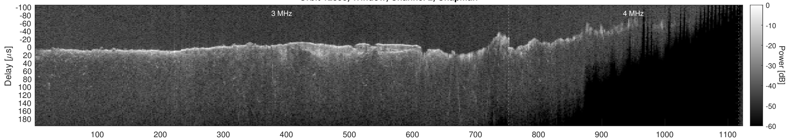
Orbit 12858, Window, Channel 2, Optimized
