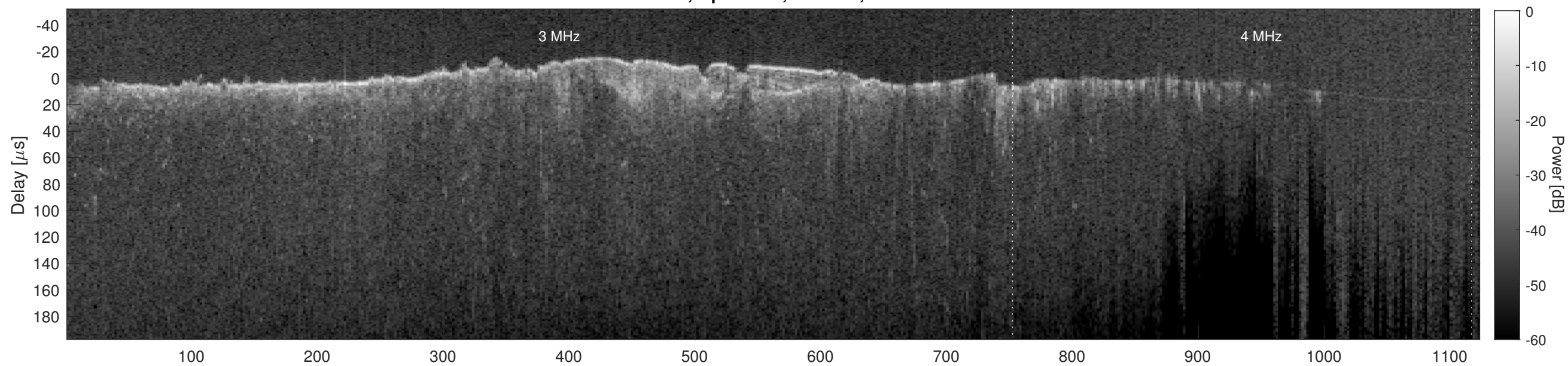
Orbit 12858, Cluttergram
