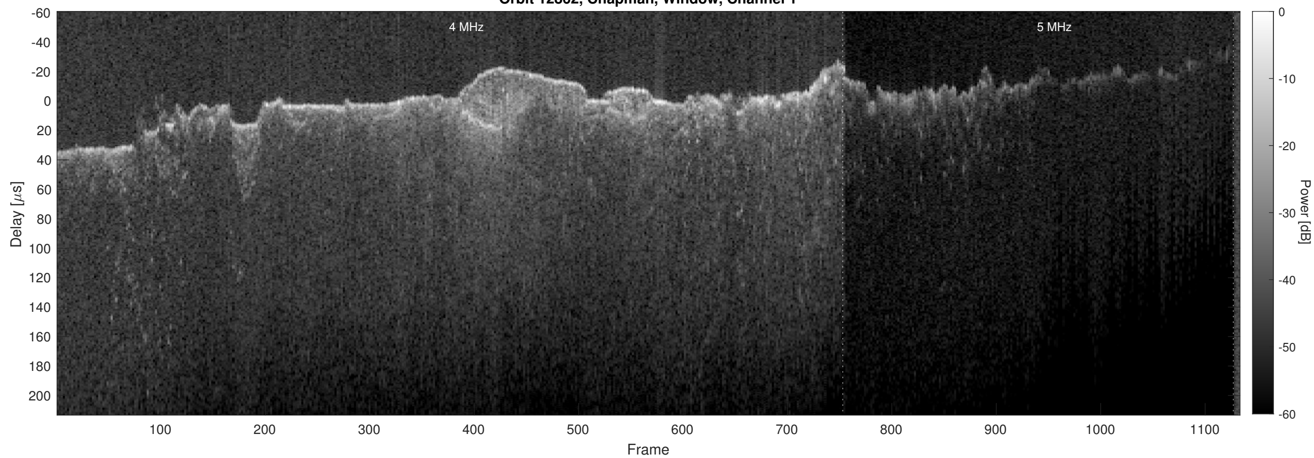
Orbit 12862, Chapman, Window, Channel 2
