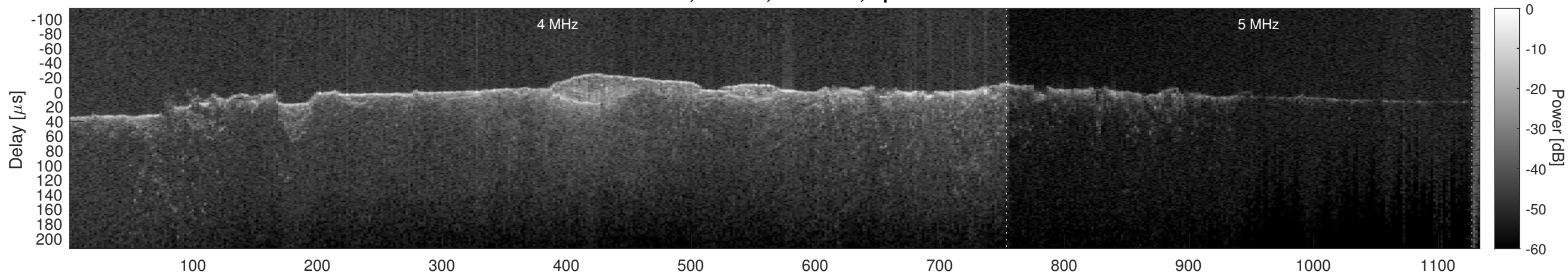
Orbit 12862, Cluttergram
