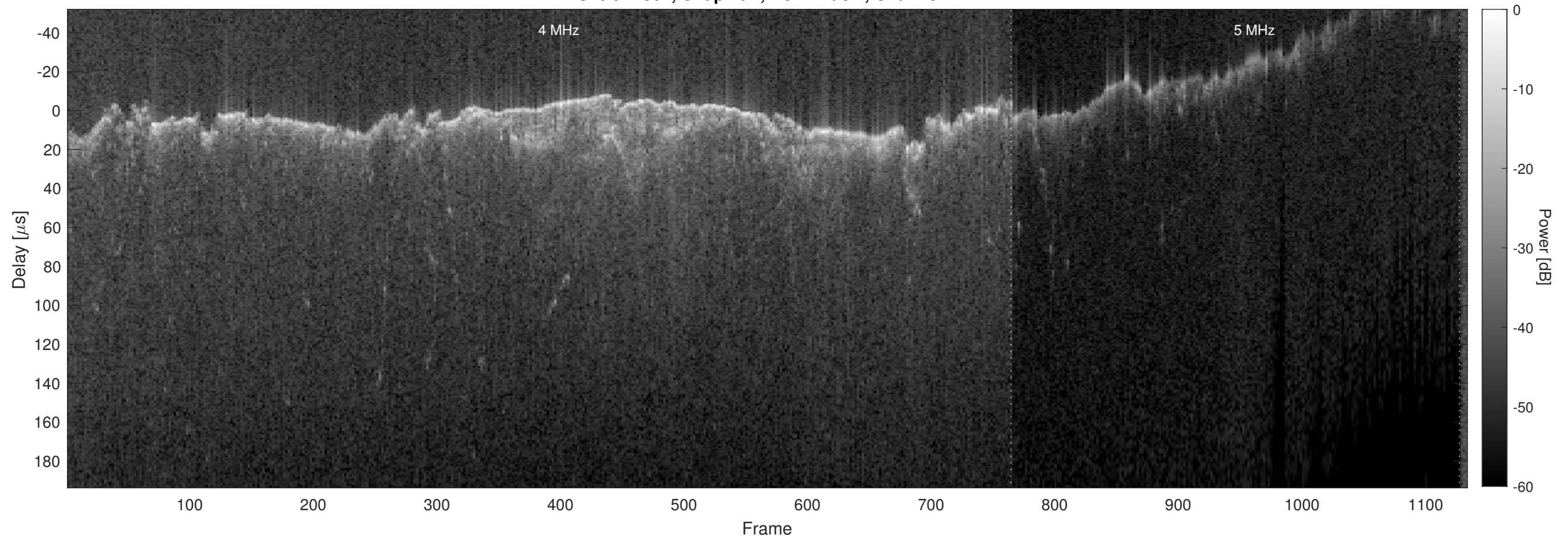
Orbit 12864, Chapman, No Window, Channel 2
