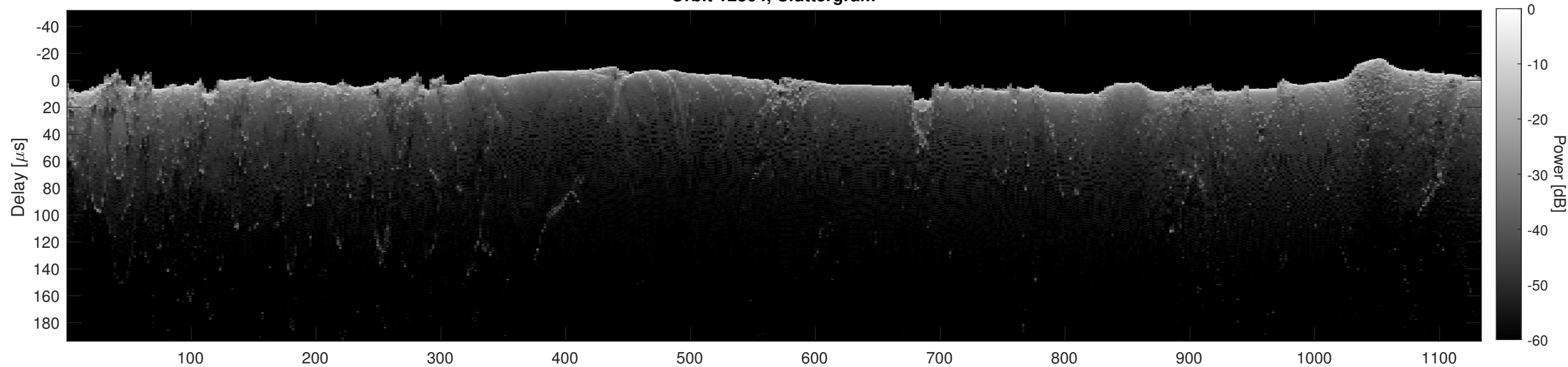
Orbit 12864, Cluttergram
