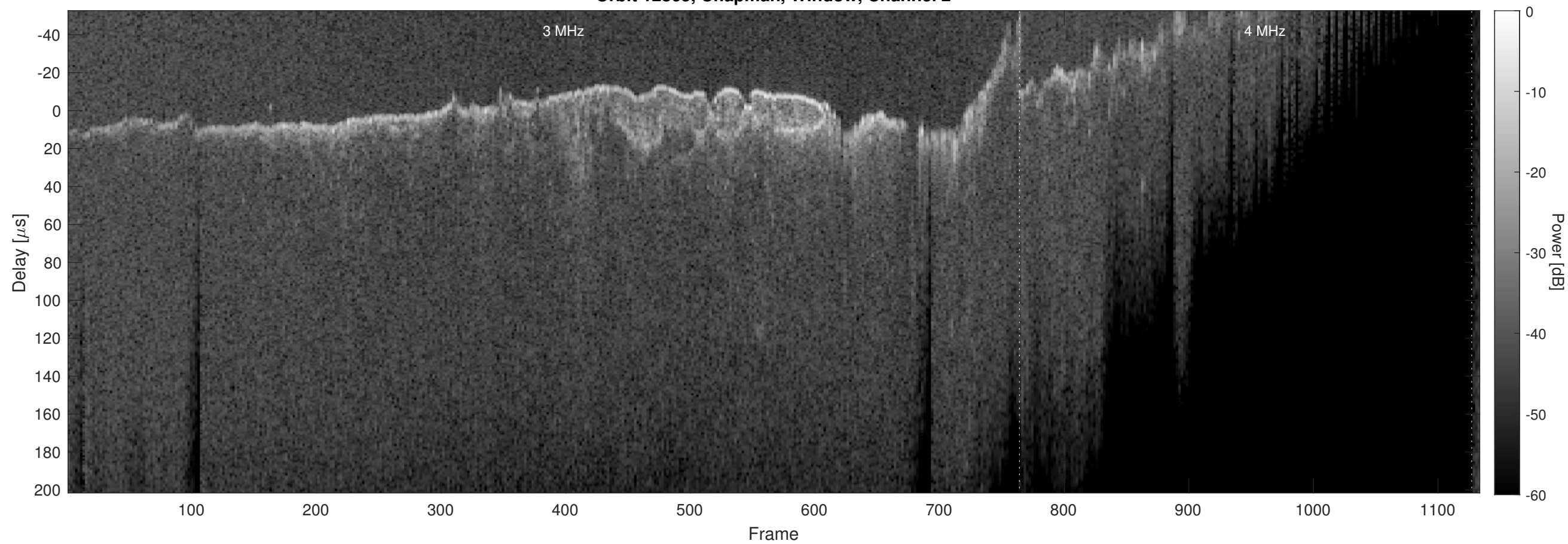
Orbit 12865, Chapman, Window, Channel 2
