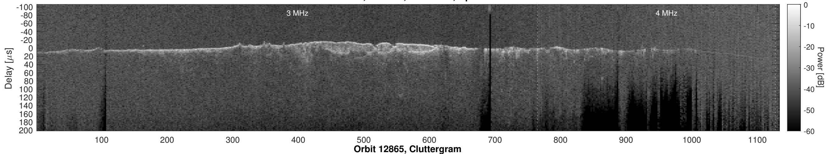
Orbit 12865, Window, Channel 2, Optimized
