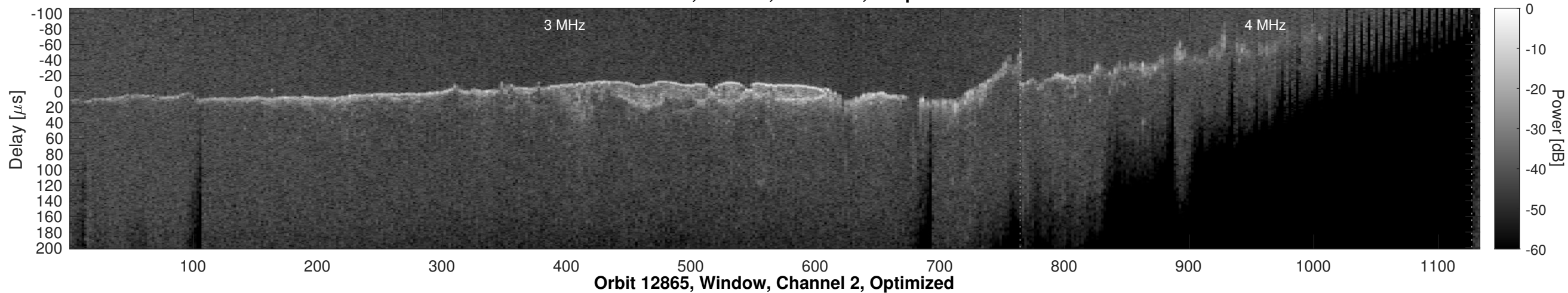
Orbit 12865, Window, Channel 2, Chapman
