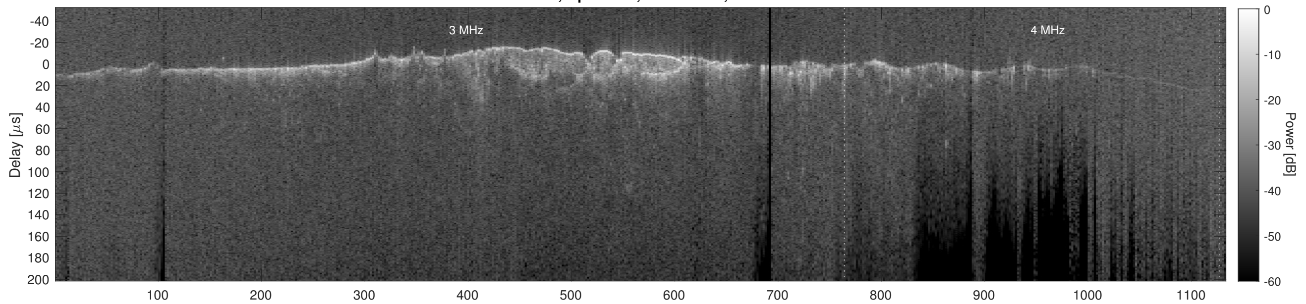
Orbit 12865, Cluttergram
