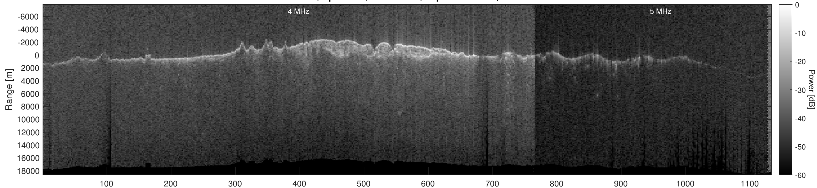
Orbit 12865, Optimized, No Window, Depth-Corrected, Channel 2
