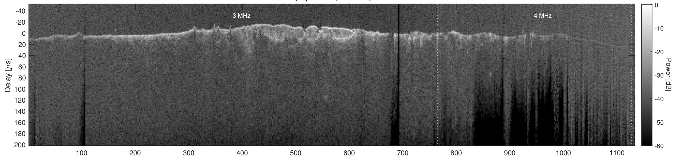
Orbit 12865, Cluttergram
