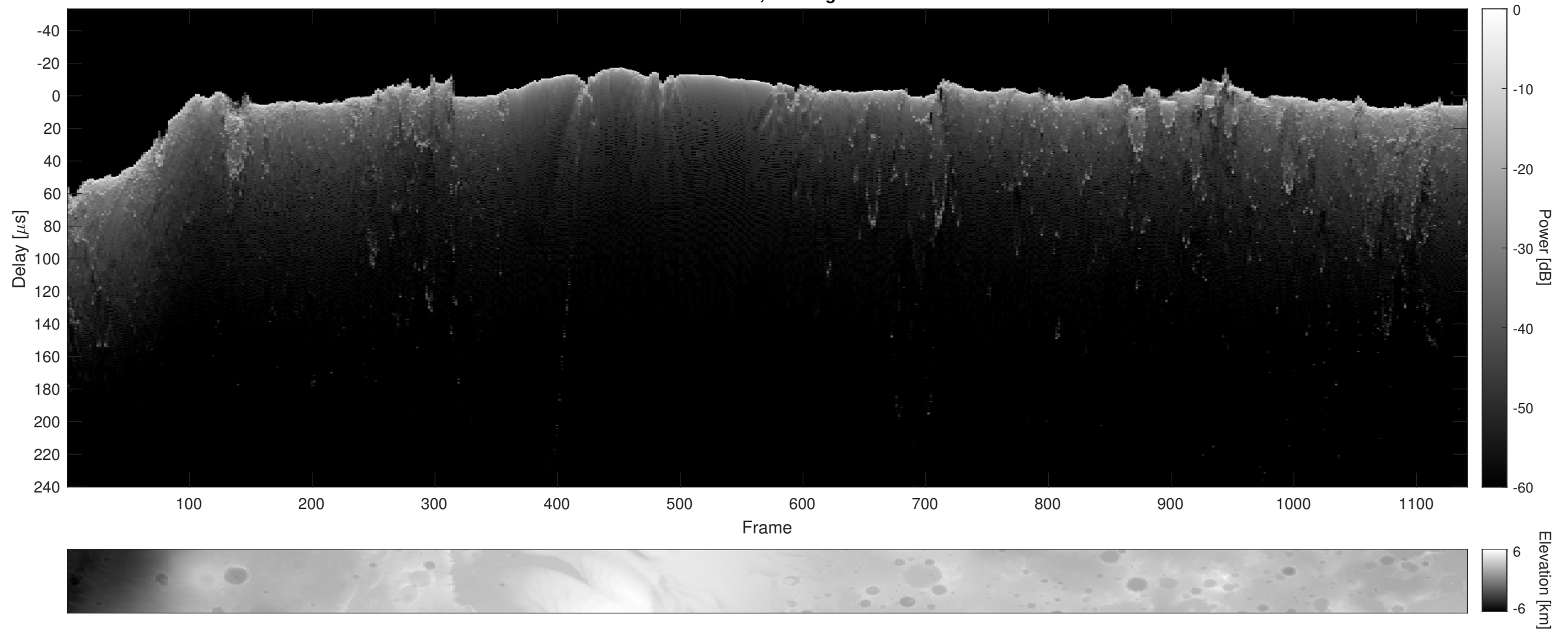
Orbit 12868, Cluttergram
