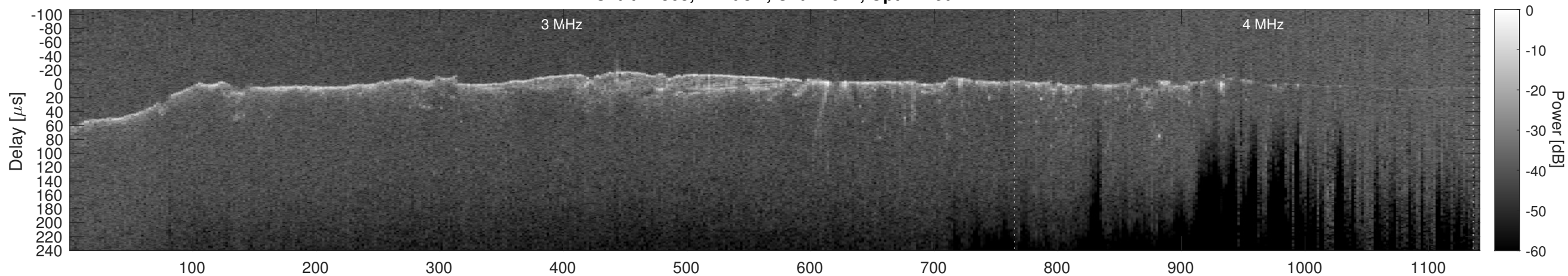
Orbit 12868, Cluttergram
