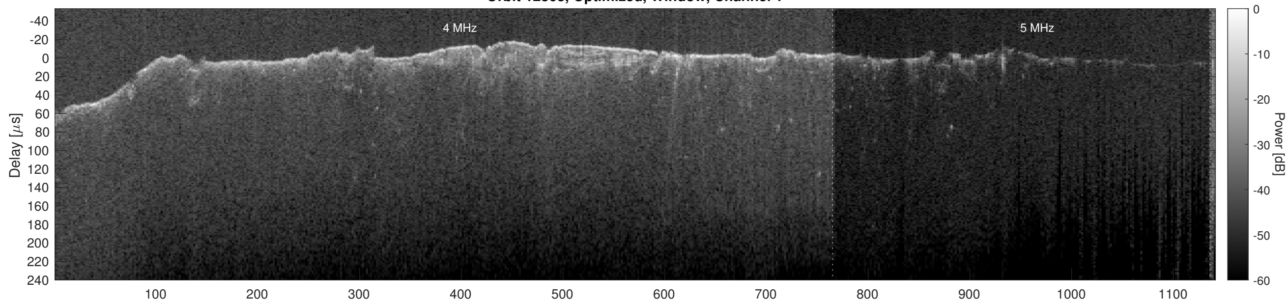
Orbit 12868, Optimized, Window, Channel 2
