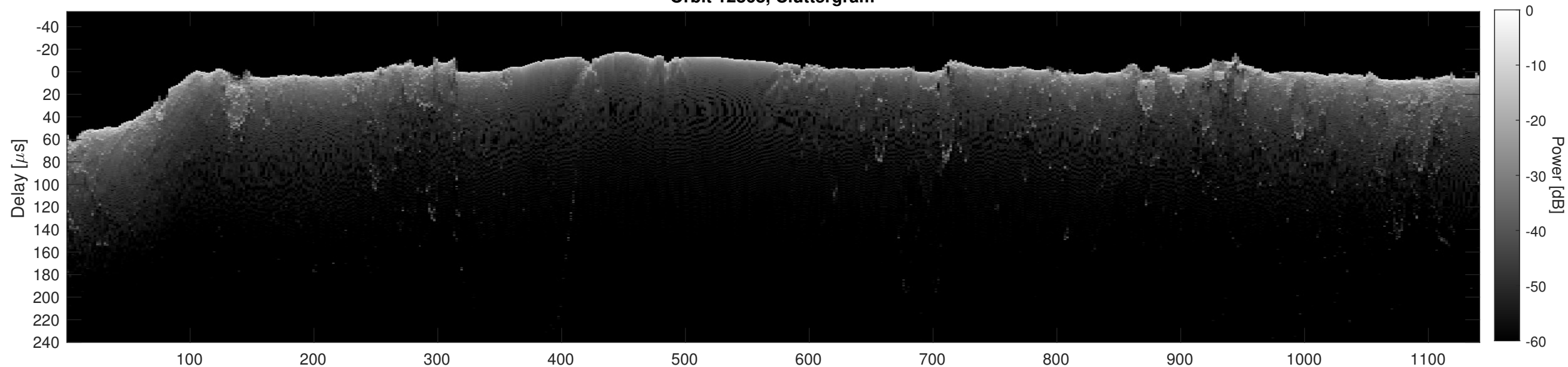
Orbit 12868, Cluttergram
