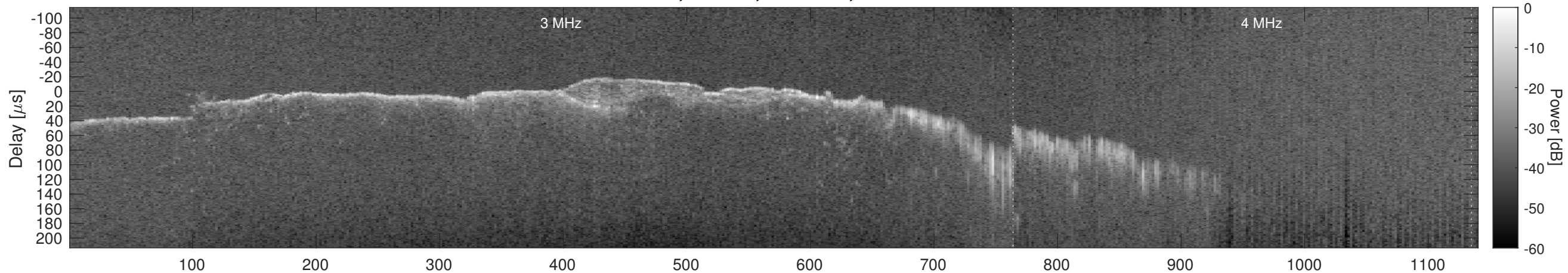
Orbit 12869, Window, Channel 2, Chapman
