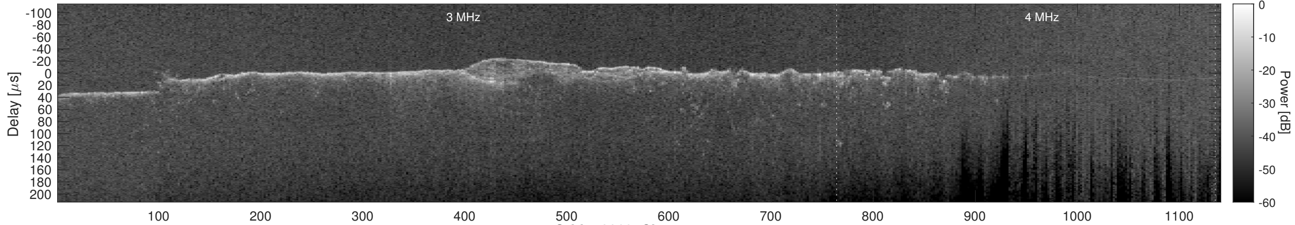
Orbit 12869, Cluttergram
