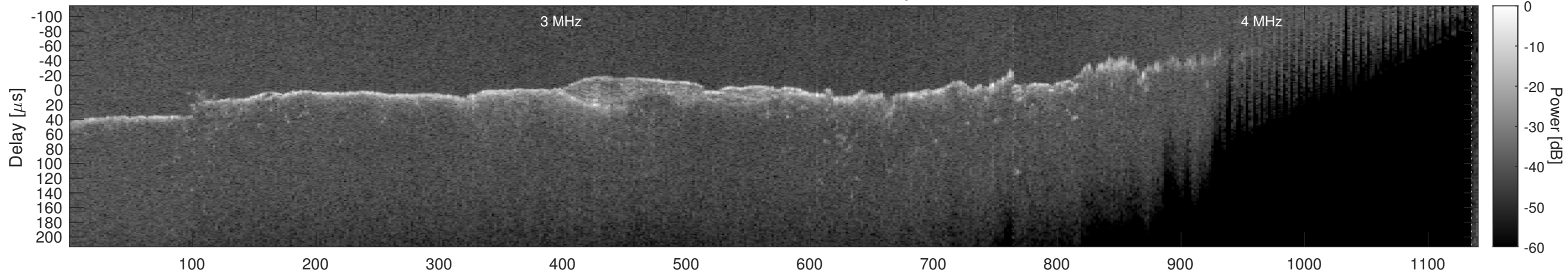
Orbit 12869, Window, Channel 2, Optimized
