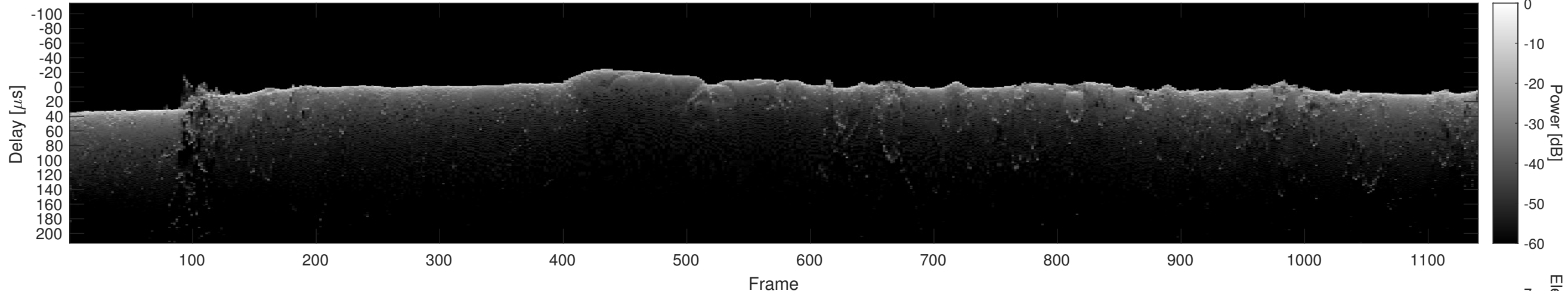
Orbit 12869, Cluttergram
