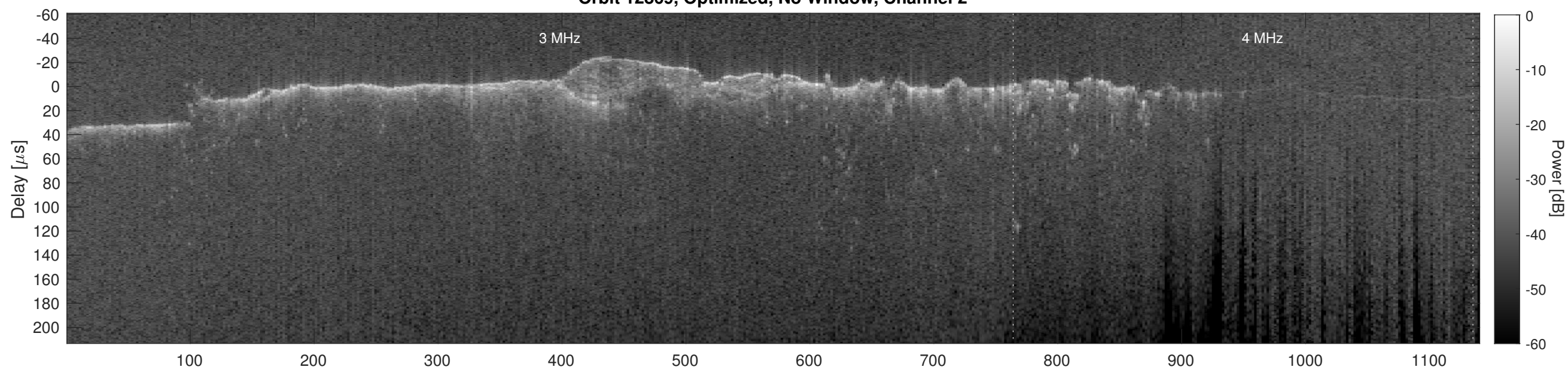
Orbit 12869, Cluttergram
