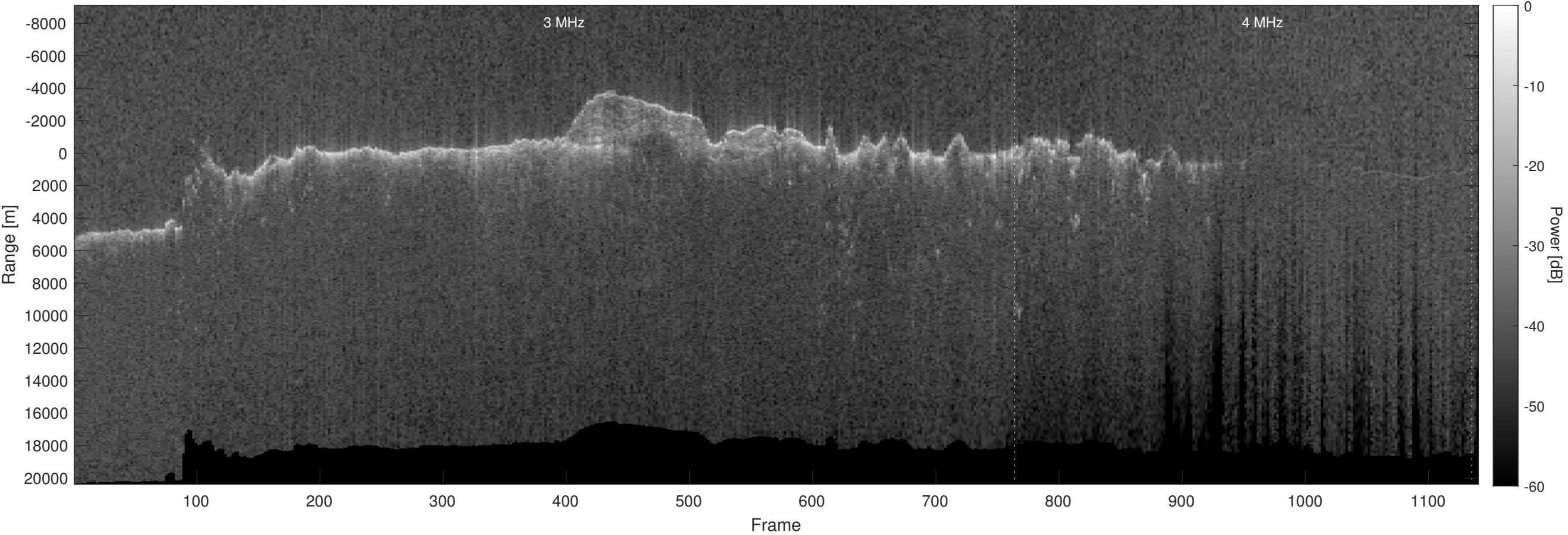
Orbit 12869, Optimized, No Window, Depth-Corrected, Channel 2
