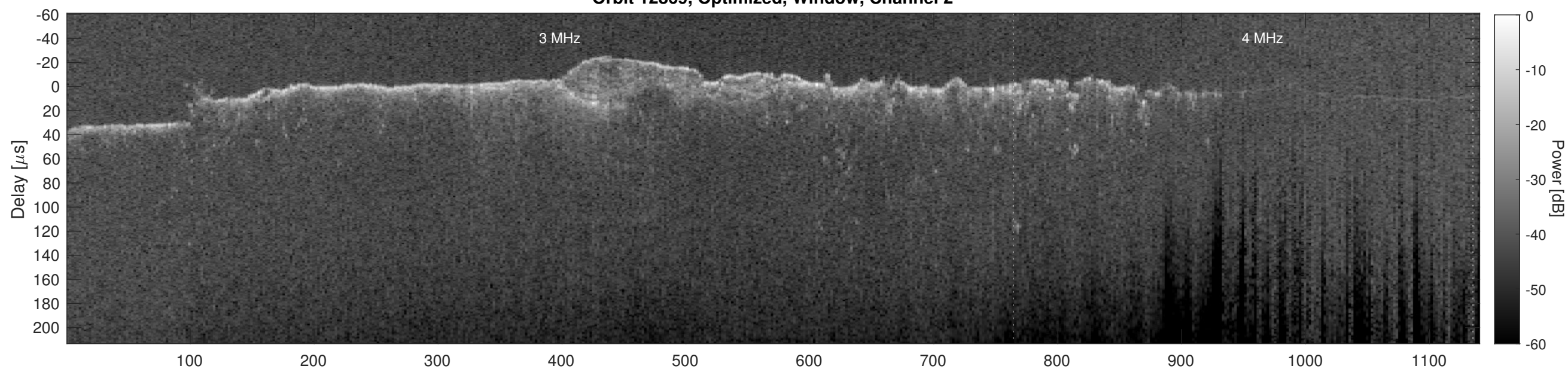
Orbit 12869, Cluttergram
