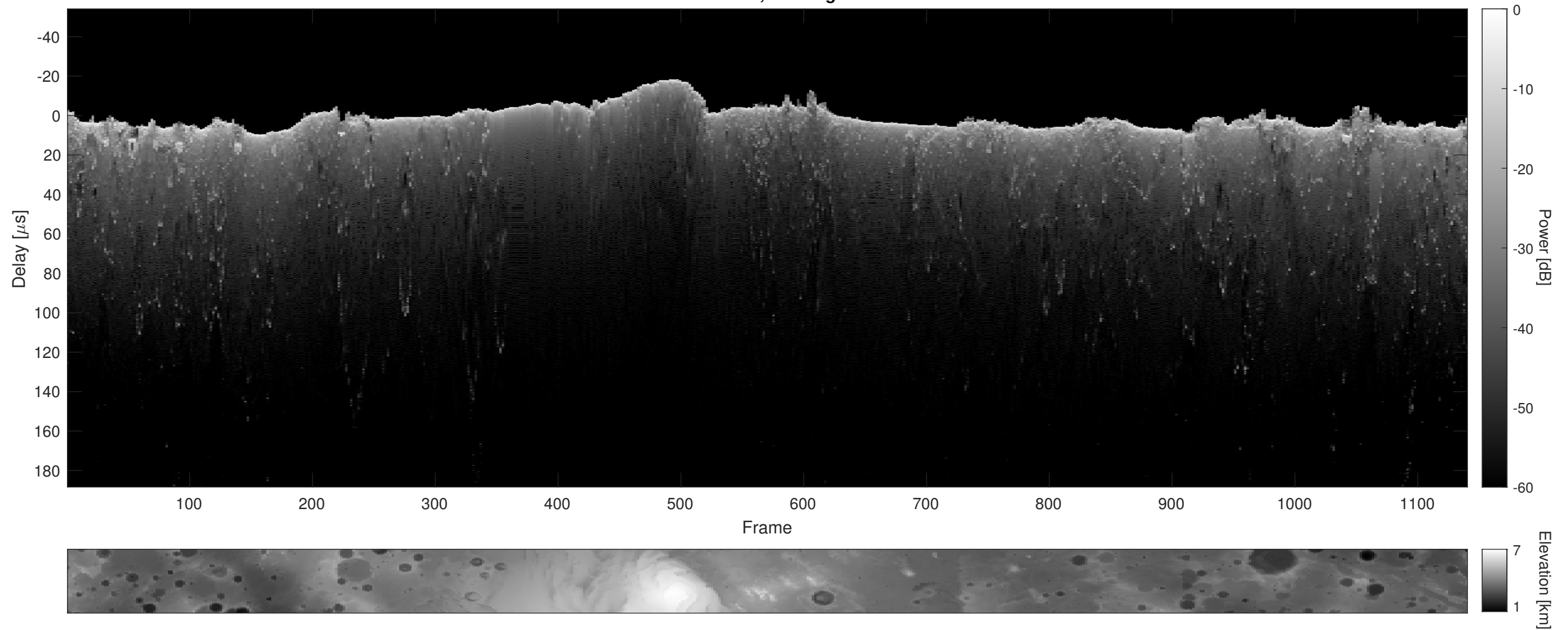
Orbit 12870, Cluttergram
