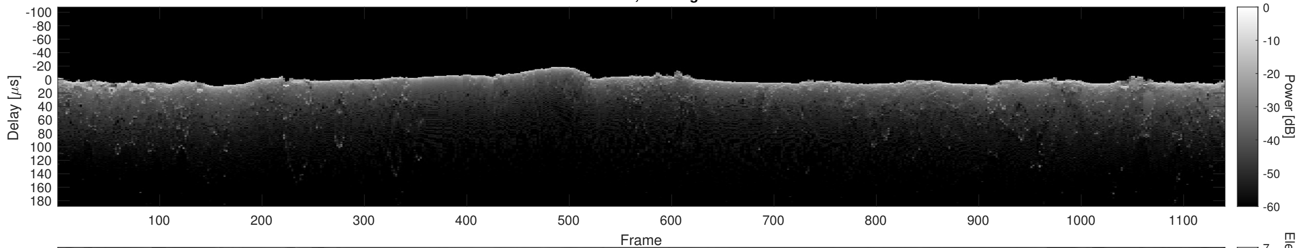
Orbit 12870, Cluttergram
