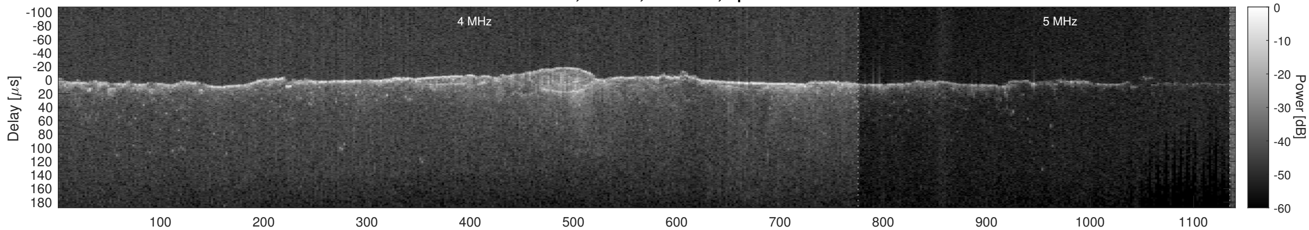
Orbit 12870, Cluttergram
