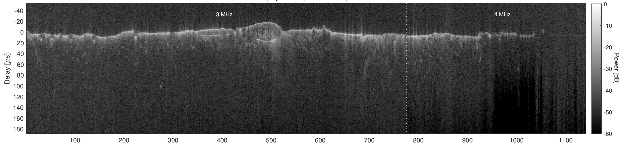
Orbit 12870, Cluttergram
