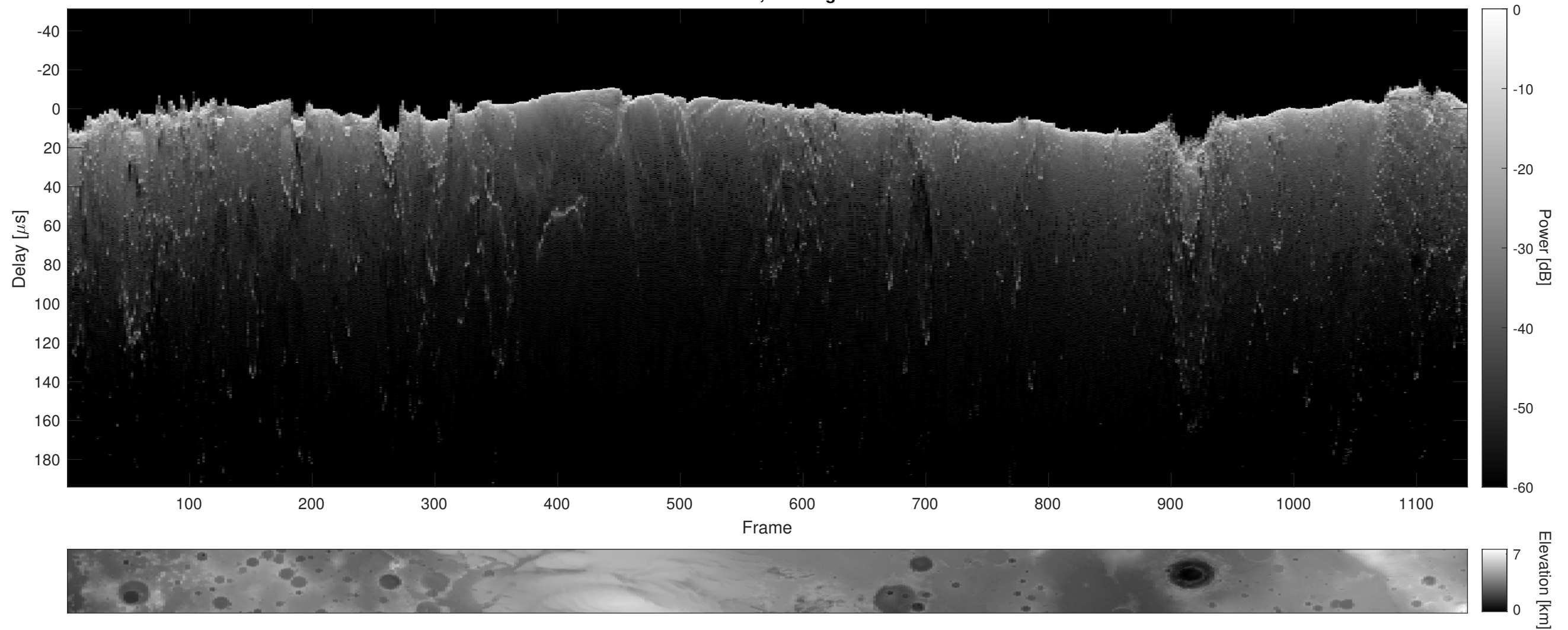
Orbit 12871, Cluttergram
