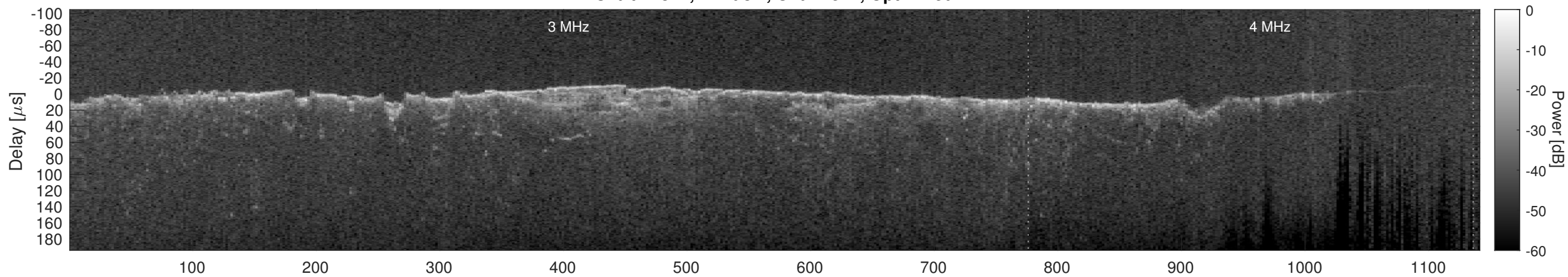
Orbit 12871, Cluttergram
