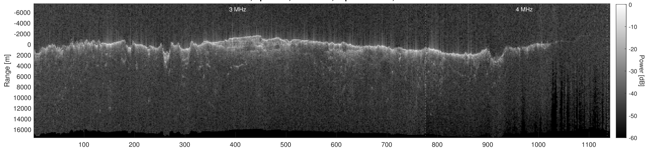
Orbit 12871, Depth-Corrected Cluttergram
