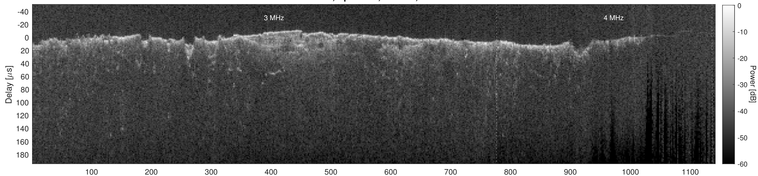
Orbit 12871, Cluttergram
