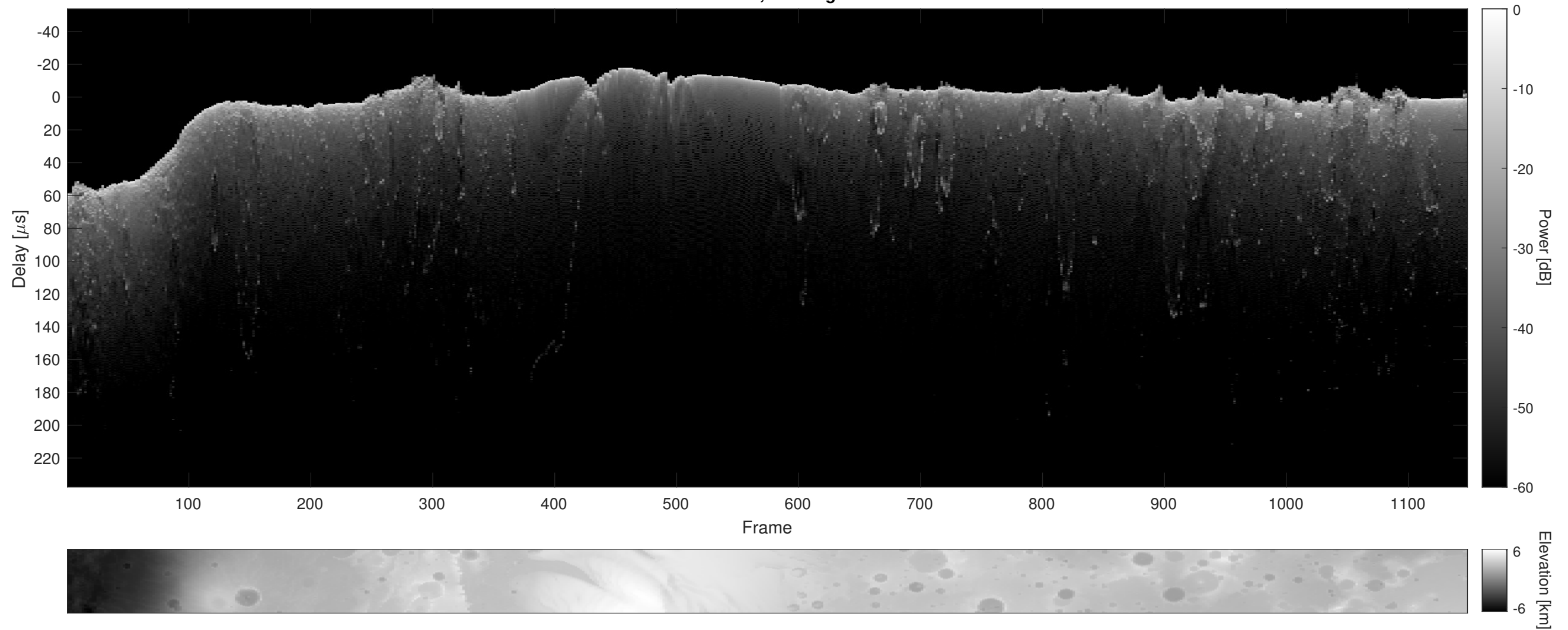
Orbit 12875, Cluttergram
