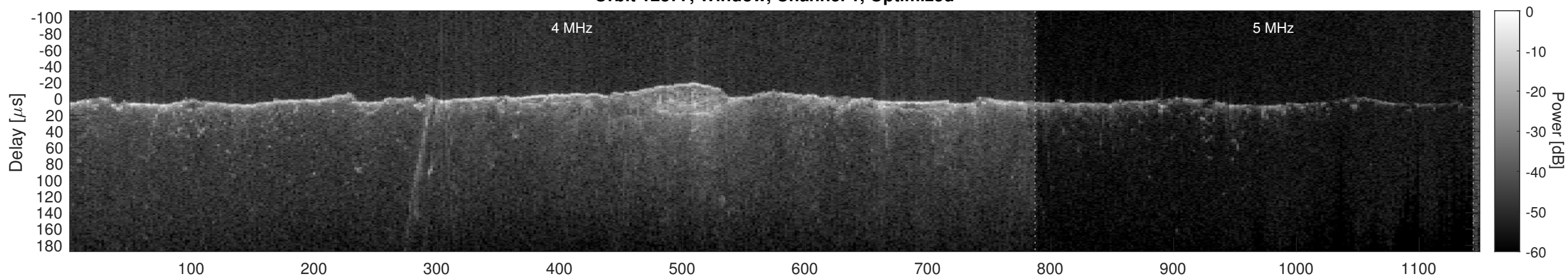
Orbit 12877, Cluttergram
