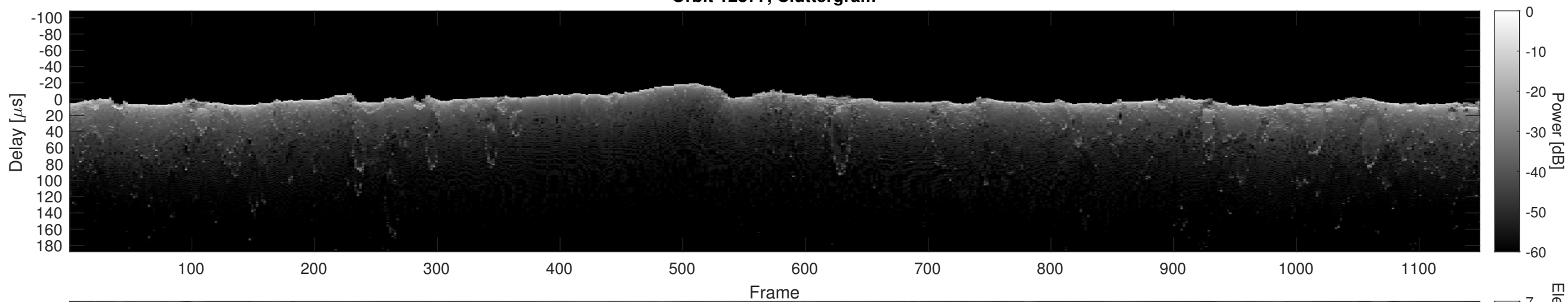
Orbit 12877, Cluttergram
