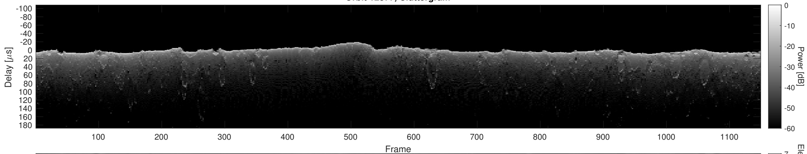
Orbit 12877, Cluttergram
