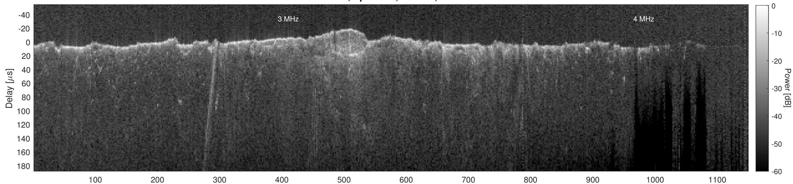
Orbit 12877, Cluttergram
