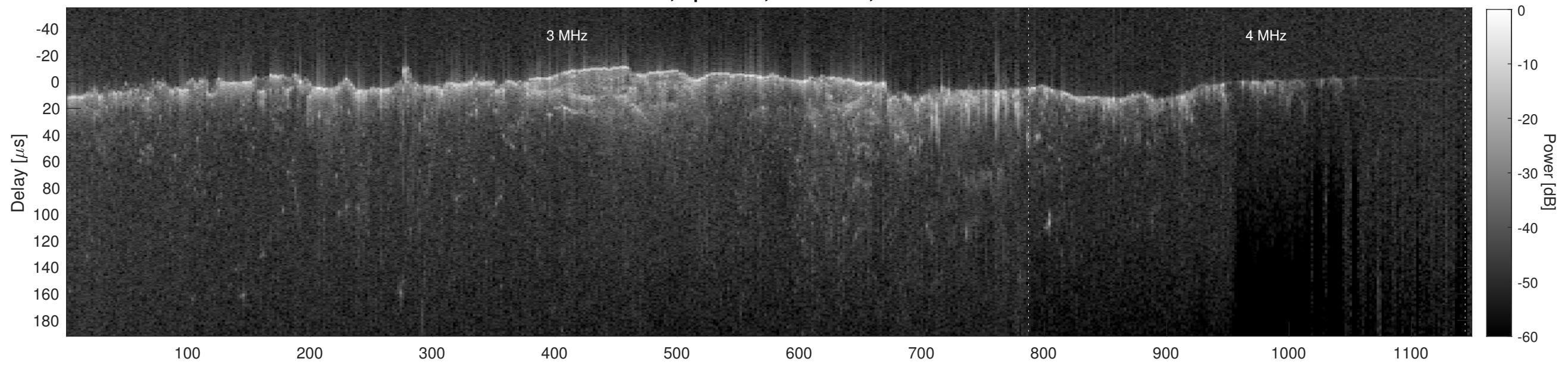
Orbit 12878, Cluttergram
