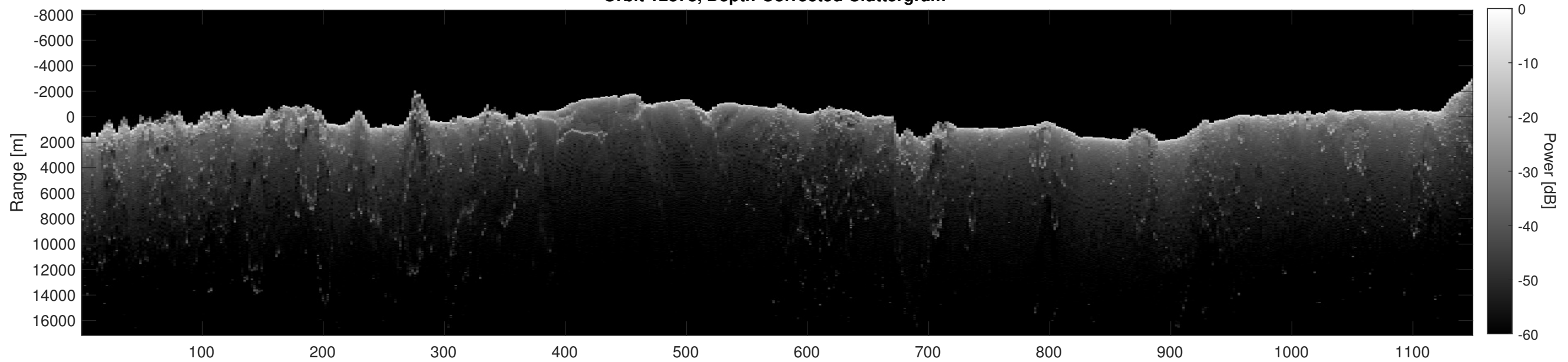
Orbit 12878, Depth-Corrected Cluttergram
