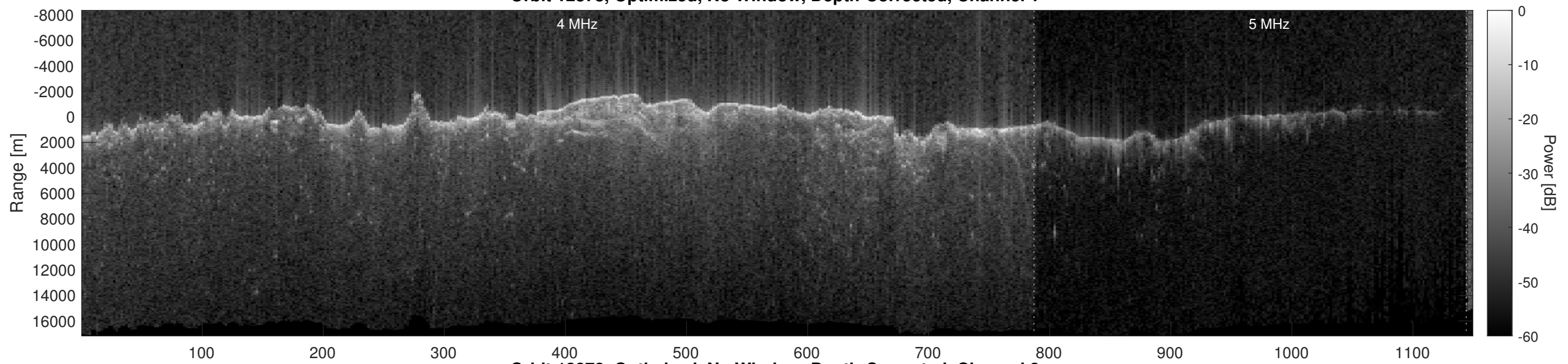
Orbit 12878, Optimized, No Window, Depth-Corrected, Channel 2
